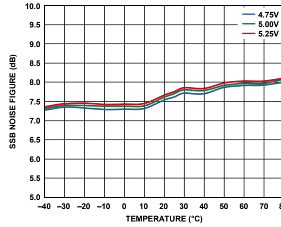
Figure 12. SSB Noise Figure vs. Temperature
