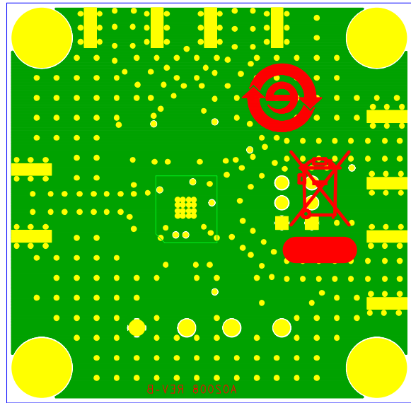
Figure 54. Evaluation Board Bottom Layer
