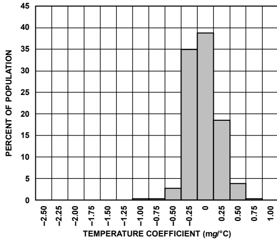
Figure 9. X-Axis Zero g Bias Temperature Coefficient, V_s = 3\text{ V}
