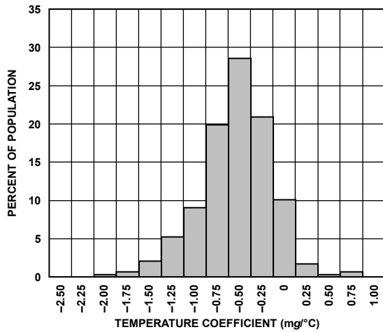
Figure 10. Y-Axis Zero g Bias Temperature Coefficient, V_s = 3\text{ V}
