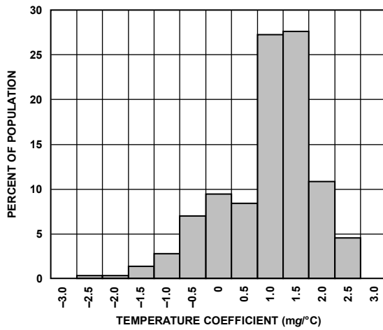
Figure 11. Z-Axis Zero g Bias Temperature Coefficient, V_s = 3\text{ V}
