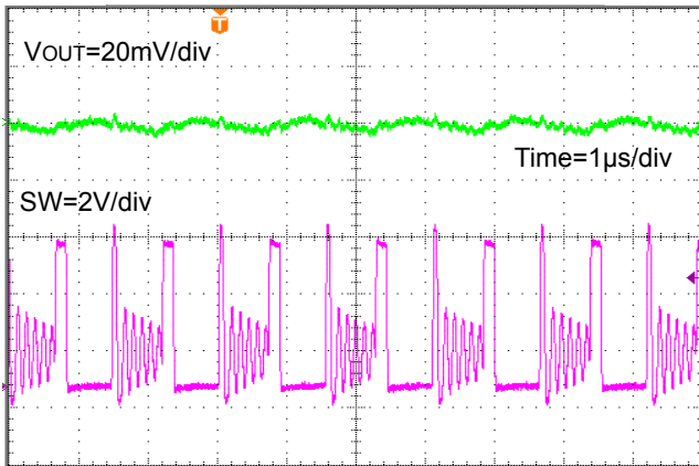
Figure 32. Switching Waveform (V IN =5V, V OUT =1.2V, FREQ=L, I OUT =0.1A)
