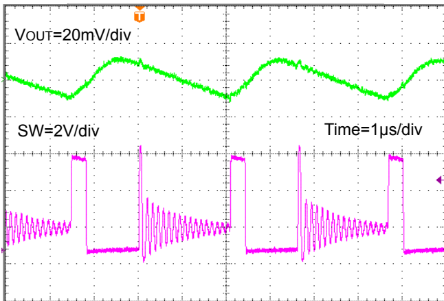
Figure 34. Switching Waveform (V IN =5V, V OUT =1.2V, FREQ=H, I OUT =0.2A)
