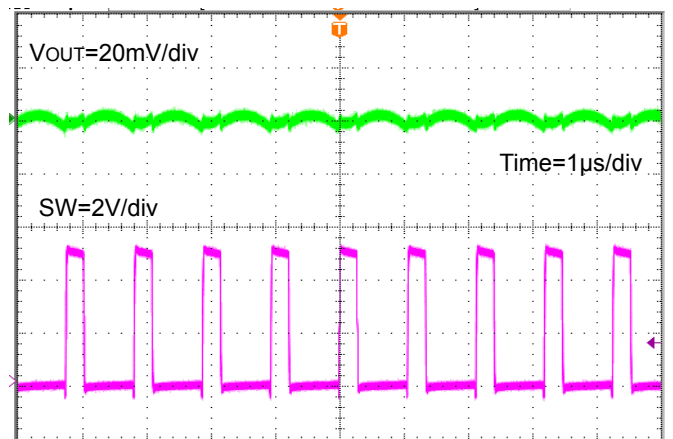
Figure 35. Switching Waveform (V IN =5V, V OUT =1.2V, FREQ=H, I OUT =2A)
