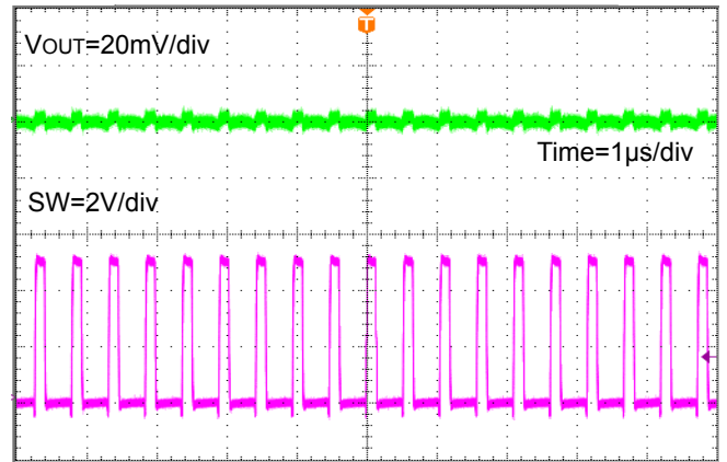
Figure 33. Switching Waveform (V IN =5V, V OUT =1.2V, FREQ=L, I OUT =2A)
