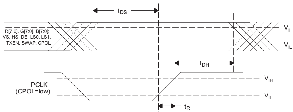
Figure 8. Setup/Hold Time
