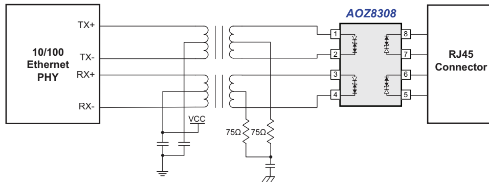
Figure 1. 10/100 Ethernet Port Connection
