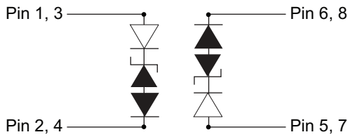
Figure 2. Circuit Diagram
