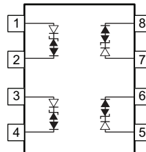
SO-8 (Top View)
