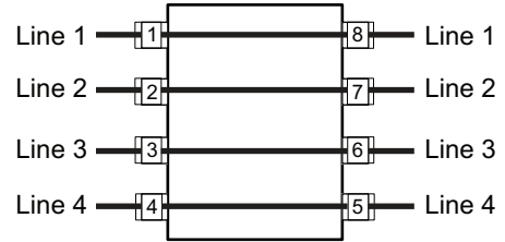
Figure 3. Low Capacitance Protection of Two Differential Line Pairs
