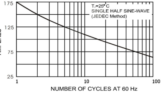
FIG. 2 - MAXIMUN NON-REPETITIVE PEAK FORWARD SURGE CURRENT PER LEG
