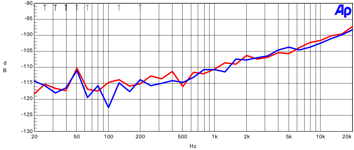
Figure 5. Crosstalk
