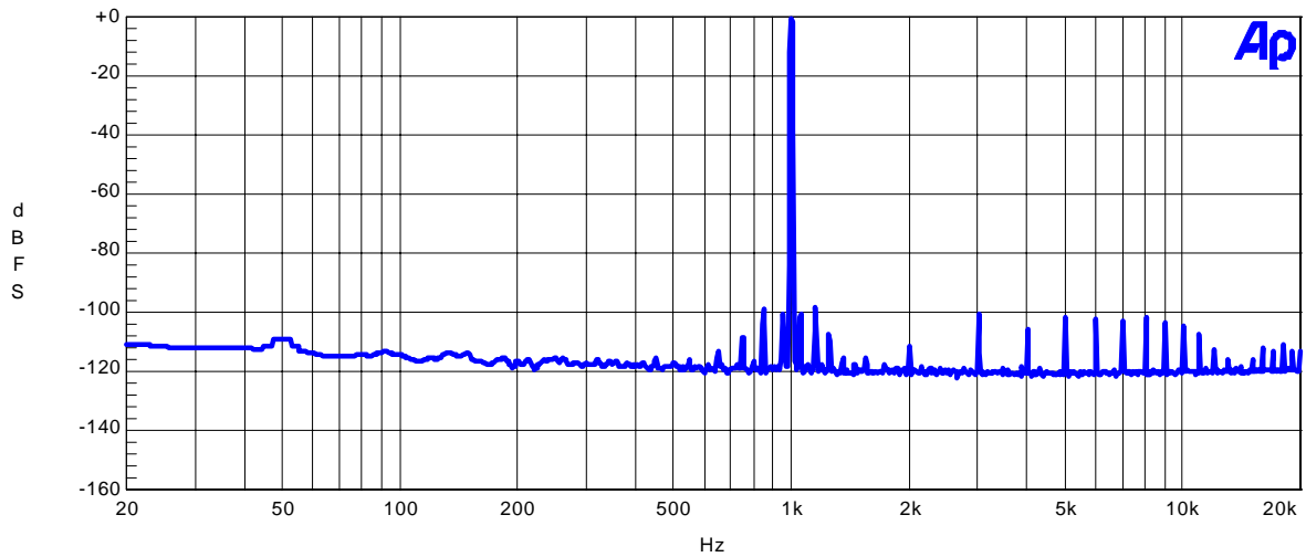
Figure 6. FFT Plot
