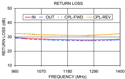
SYBD-20-142HP+ RETURN LOSS
