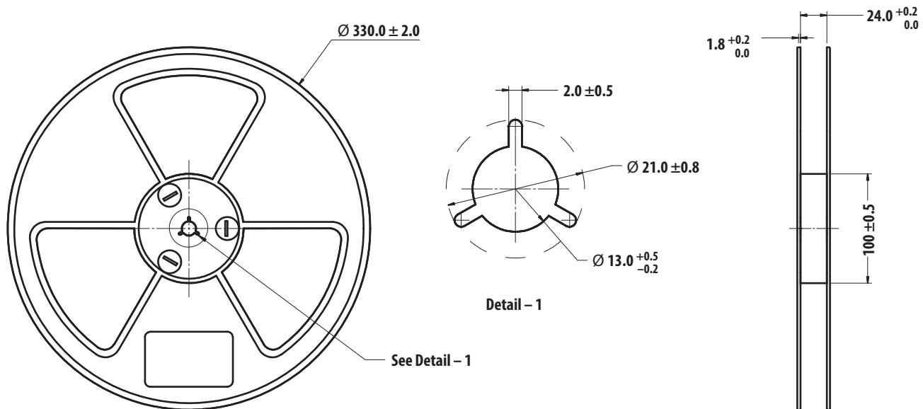
Figure 32 Reel Dimensions
