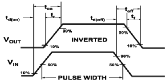
Figure 2: Switching Waveforms
