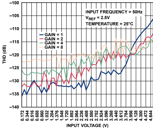
Figure 32. THD vs. Input Voltage at 2 kSPS, High Resolution Mode (Input Frequency = 50 Hz)
