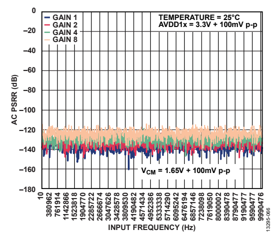
Figure 67. AC PSRR vs. Input Frequency at 2 kSPS, Low Power Mode, AVDD1x = 3.3 V + 100 mV p-p
