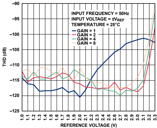
Figure 33. THD vs. Reference Voltage at 8 kSPS, High Resolution Mode (Input Frequency = 50 Hz)
