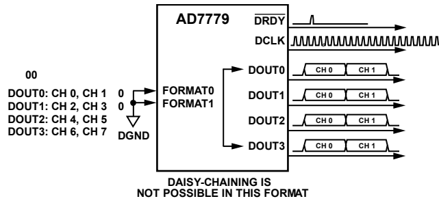
Figure 111. FORMATx Pin Configuration—FORMAT0 = 0, FORMAT1 = 0
