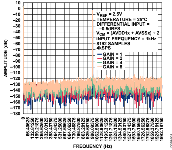
Figure 30. FFT Plot, Low Power Mode, Input Frequency ( f_{IN} ) = 1 kHz, 8192 Samples, AVSSx
