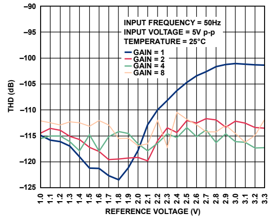
Figure 36. THD vs. Reference Voltage at 2 kSPS, Low Power Mode (Input Frequency = 50 Hz)
