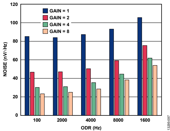
Figure 22. Noise vs. ODR, High Resolution Mode
