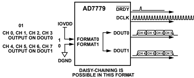
Figure 112. FORMATx Pin Configuration—FORMAT0 = 1, FORMAT1 = 0
