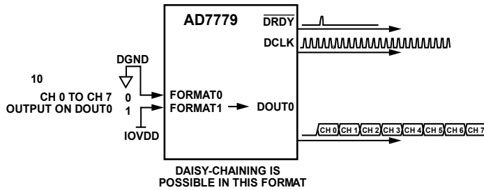
Figure 113. FORMATx Pin Configuration—FORMAT0 = 0, FORMAT1 = 1
