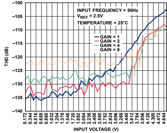
Figure 35. THD vs. Input Voltage at 500 SPS, Low Power Mode
