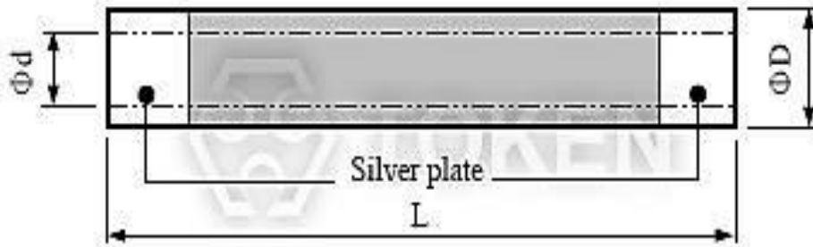
Tubular High Voltage Resistors (RMCD) Dimensions
