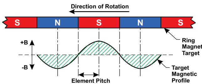
Figure 6b: Mechanical Position (Target moves past device pin 1 to pin 8)
