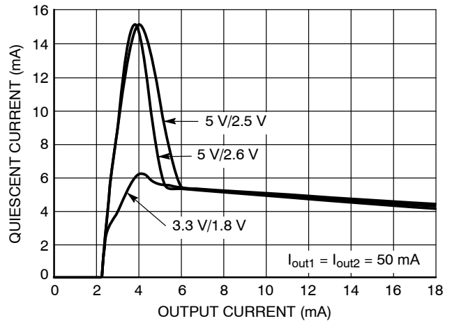
Figure 25. Quiescent Current vs. V_{IN1}
