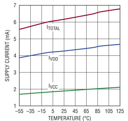
Supply Current vs Temperature (LTC6752-3)
