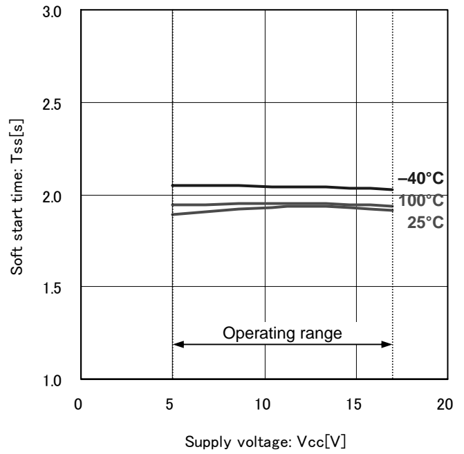
Fig.32 Soft start time
