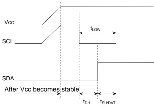
Figure 53. When SCL= 'H' and SDA= 'L'
