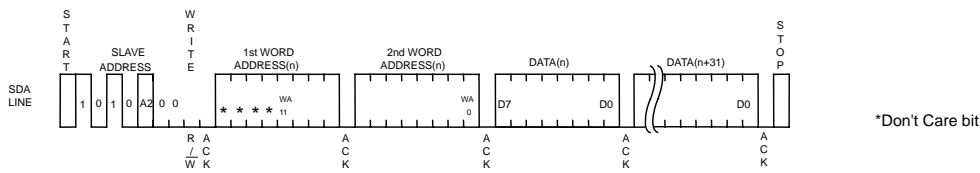
Figure 37. Page Write Cycle
