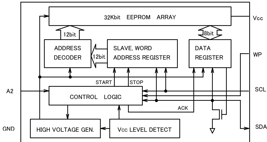
Figure 2. Block Diagram
