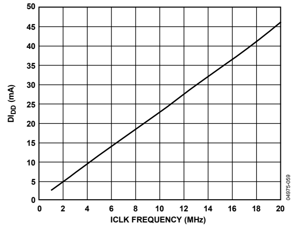
Figure 38. Decimate \times 32, D_{DD} vs. ICLK Frequency ( V_{DD} = 2.5 V)
