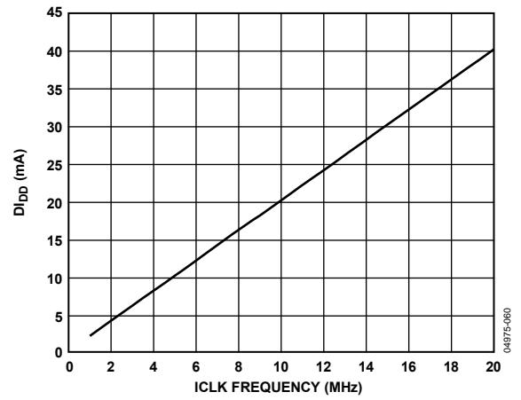
Figure 39. Decimate \times 256, D_{DD} vs. ICLK Frequency ( V_{DD} = 2.5 V)
