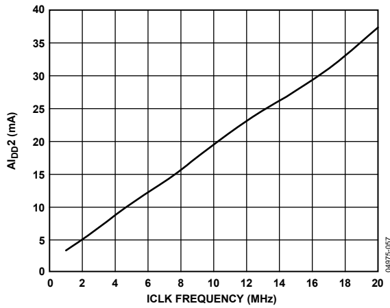
Figure 36. A_{DD2} vs. ICLK Frequency ( A_{VDD2} = 5 V)
