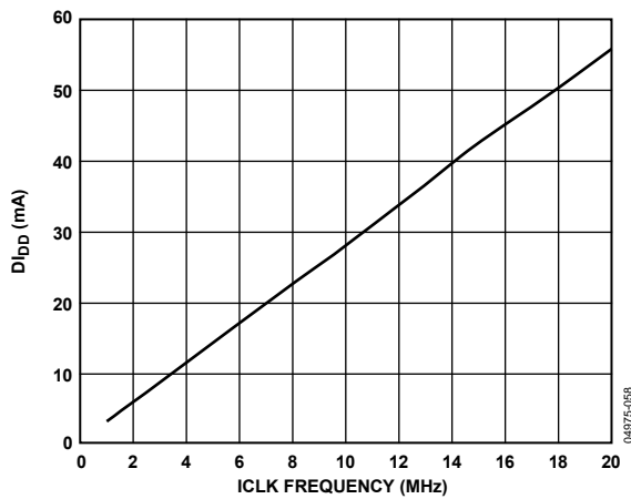
Figure 37. Decimate \times 8, D_{DD} vs. ICLK Frequency ( V_{DD} = 2.5 V)
