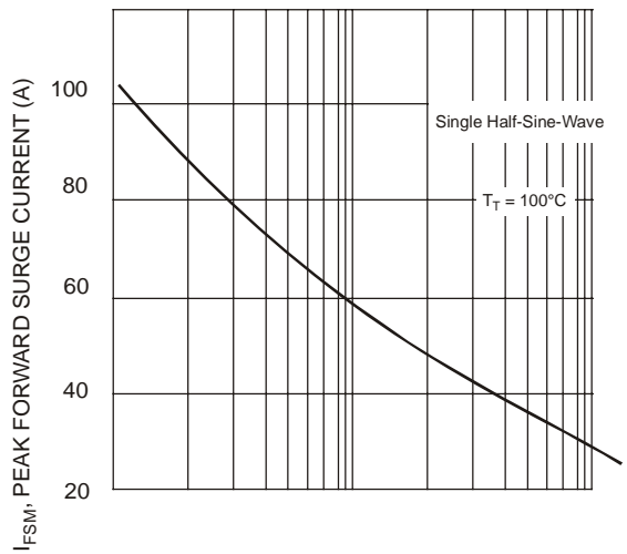
Single Half-Sine-Wave T T = 100°C
