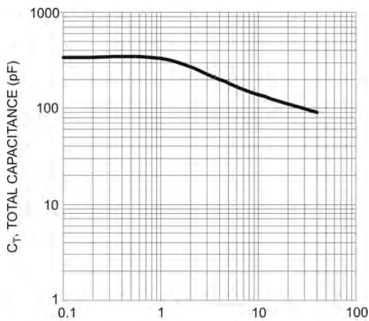
V R , REVERSE VOLTAGE (V) Fig. 5 Typical Capacitance
