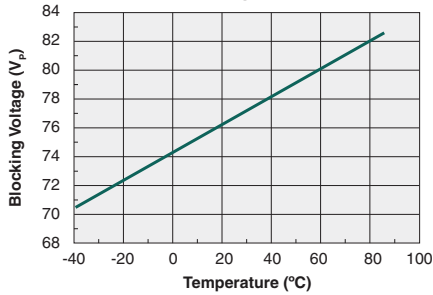
Normalized Blocking Voltage vs. Temperature
