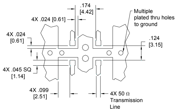
Dimensions are in Inches [Millimeters] JP503* Mounting Footprint
