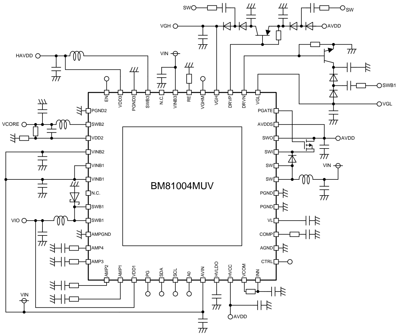
Figure 2. Application Circuit 2
