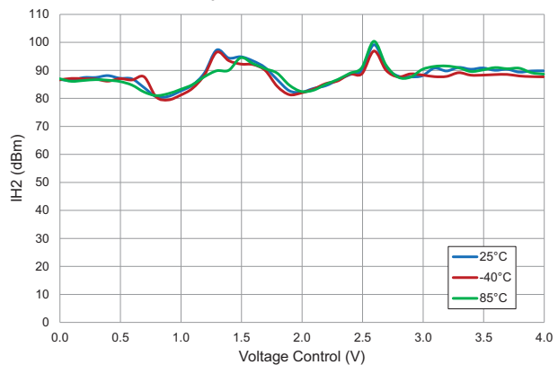
2 nd Harmonic IH 2 versus Voltage Control VCA 5V Mode, V DD =5V, F=1GHz Extrapolated from Pin=+15dBm
