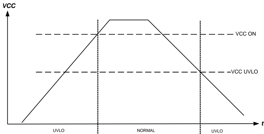
Figure 11: Vcc UVLO
