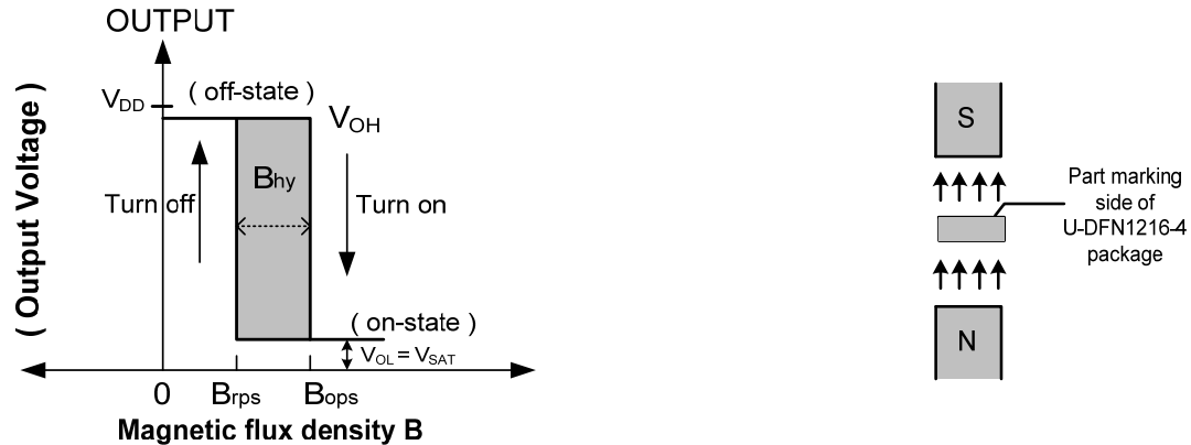
Magnetic Field Direction for Unipolar Mode Operation
