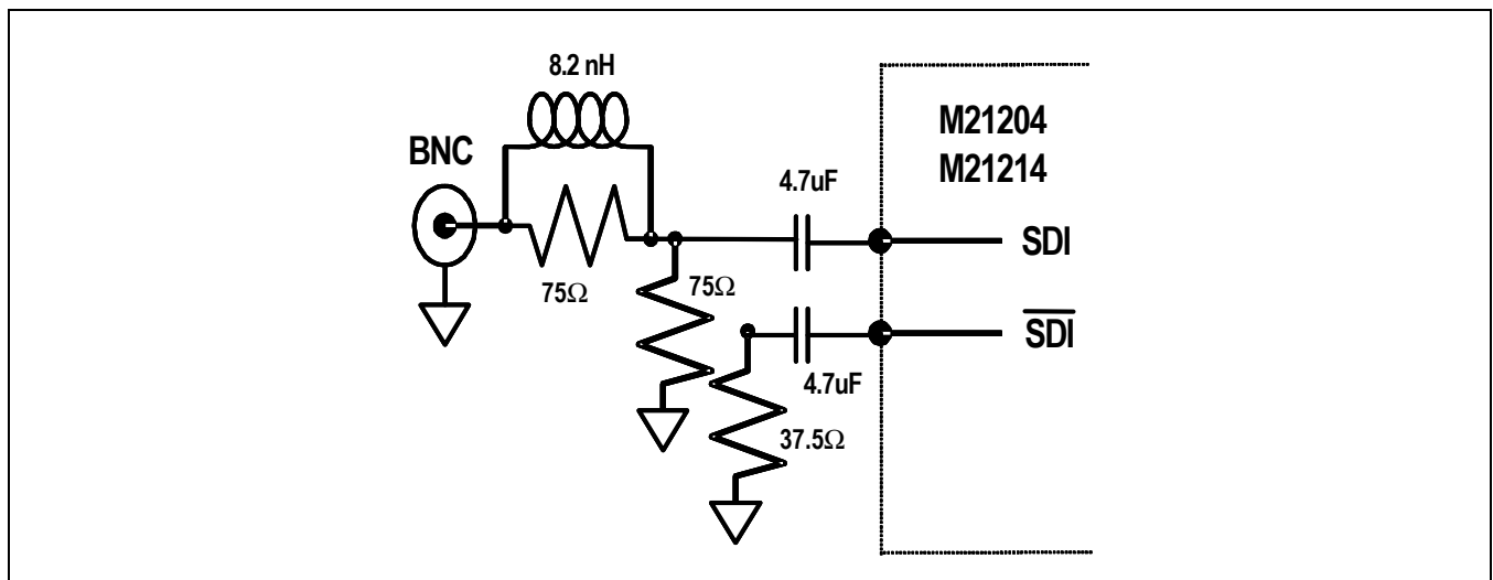
Figure 1-1. Single-ended Typical Input Matching/Termination Network
