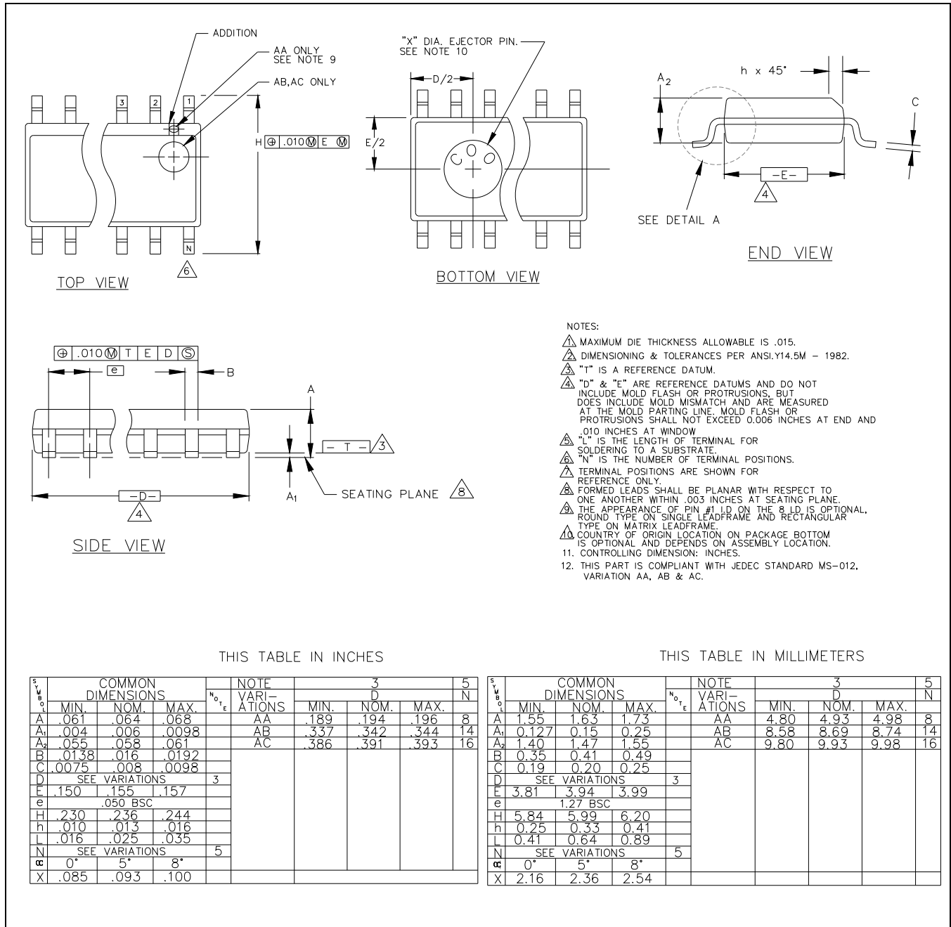
Figure 2-2. M21204/M21214 Packaging Details
