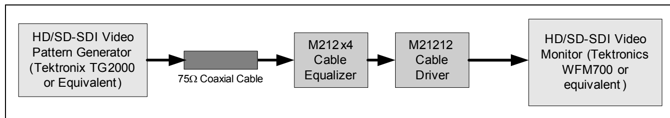
Figure 1-2. Test Setup Diagram for M21204/M21214 Cable Equalizer Evaluation
