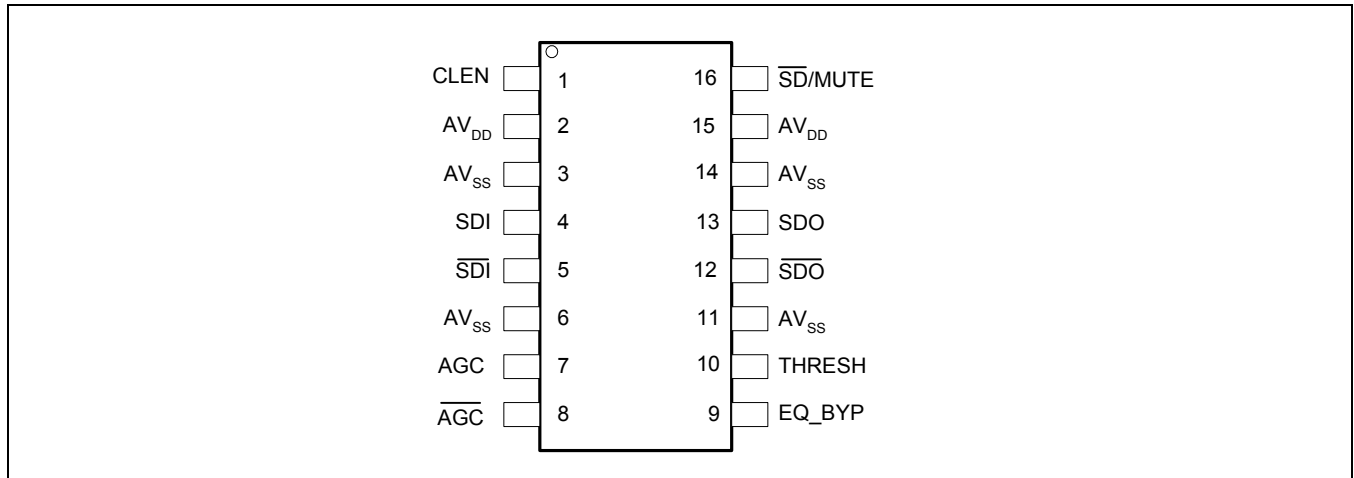
Figure 1-3. M21204/M21214 Pin Assignments
