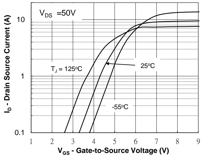
Fig.2 Transfer Characteristic
