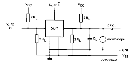
Fig. 16 Test circuit for measuring crosstalk between control and any switch.
