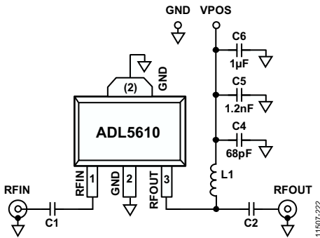
Figure 26. Basic Connections
