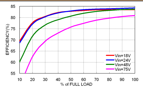
MPP03-48S05WA Efficiency vs. Output Load
