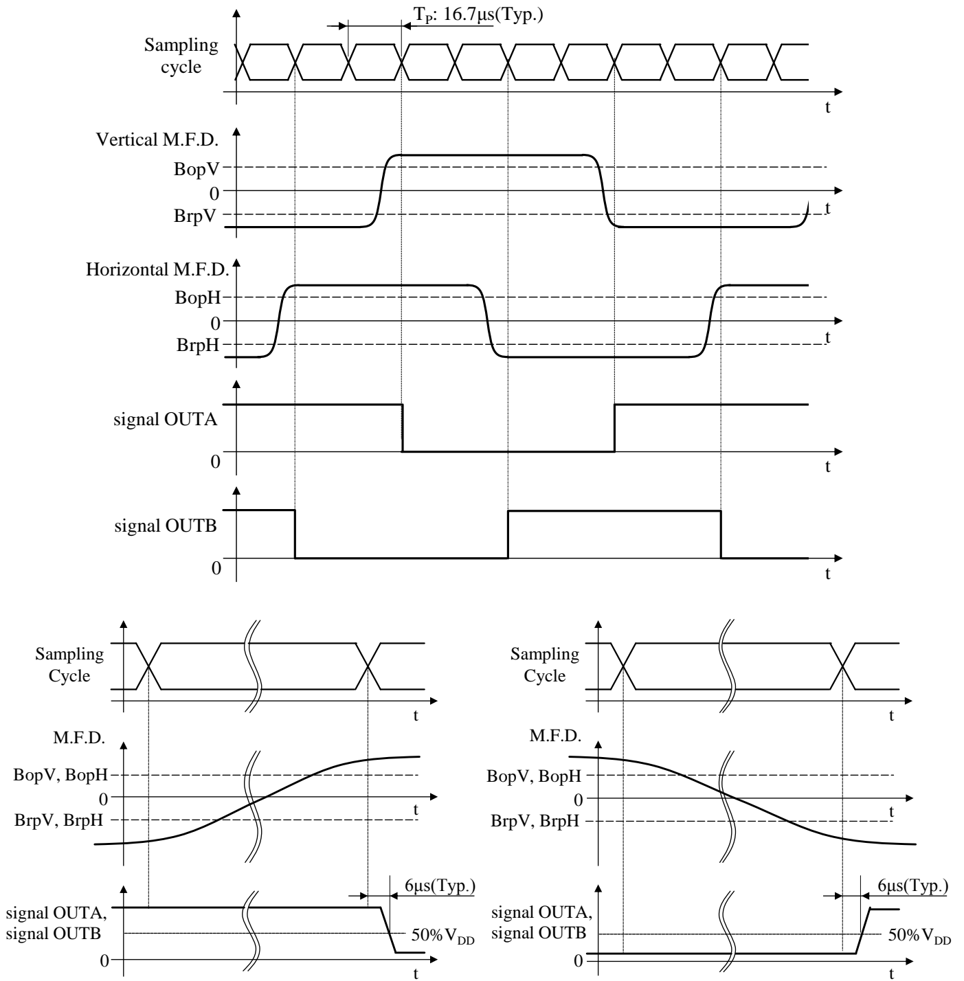
Figure 4. Timing diagram
