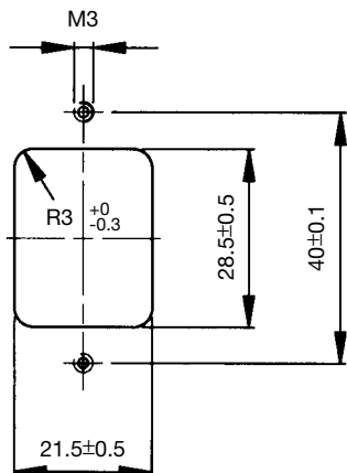
PANEL CUT-OUT
