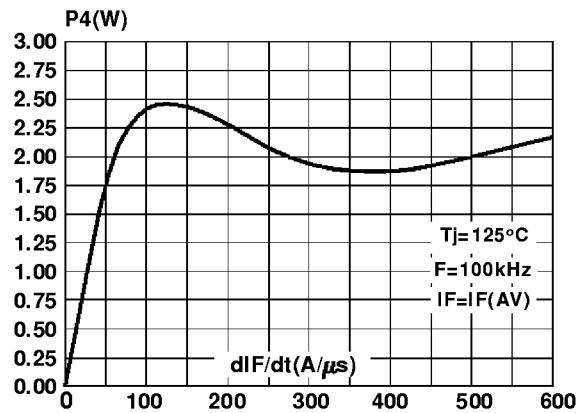
Fig 7 : Switching ON losses versus dI/dt
