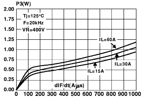
Fig 6 : Switching OFF losses versus dI/dt
