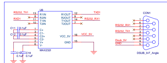
RS232
