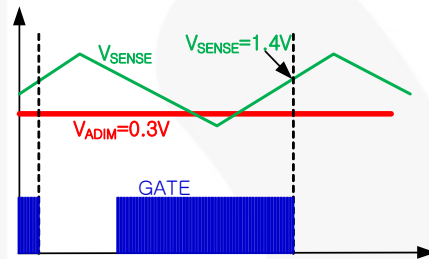
Figure 32. OCP Waveforms at V ADIM =0.3V
