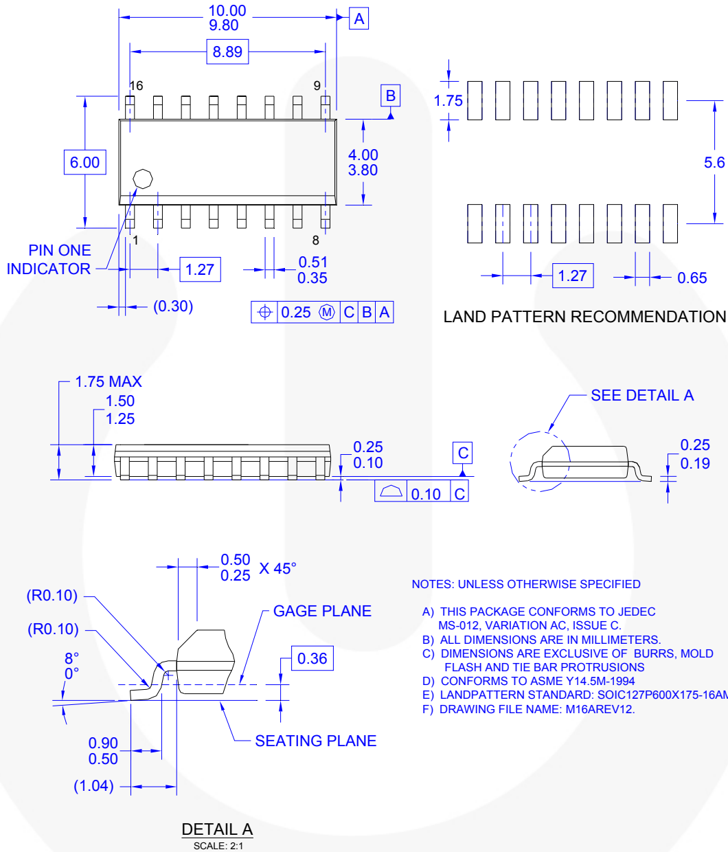
Figure 36. 16-Lead, Small Outline Integrated Circuit (SOIC)
