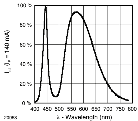
Figure 2. Relative Spectral Emission
