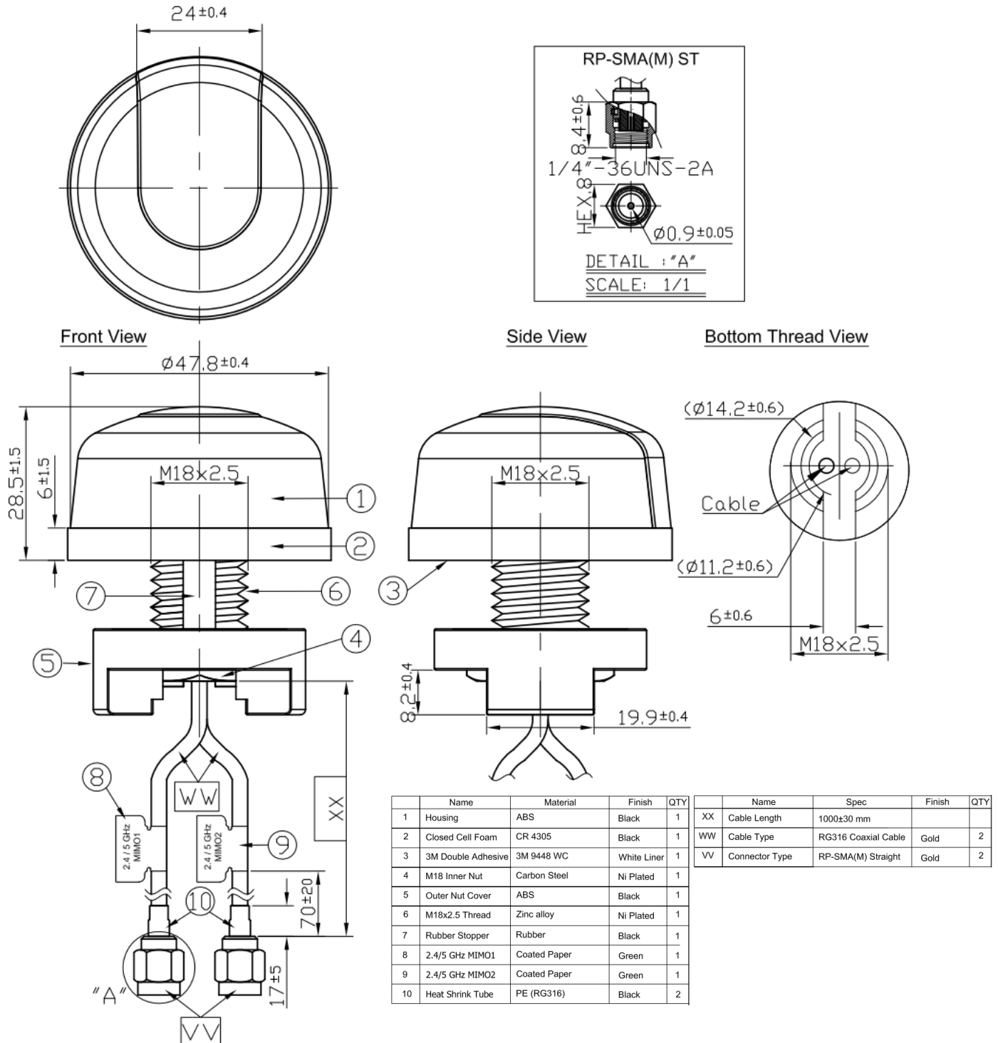
Figure 23. Antenna Drawing
