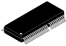
54-PIN SOICW-EP 98ASA00367D
