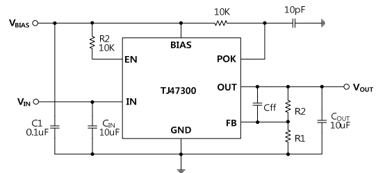
Circuit #2
