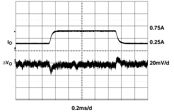
FIGURE 10. TRANSIENT RESPONSE
