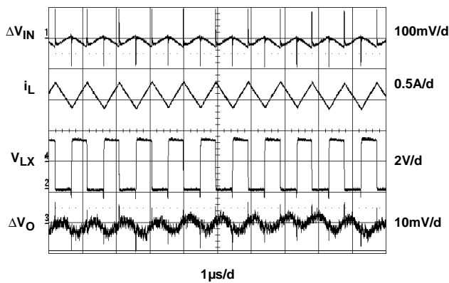
FIGURE 11. STEADY-STATE
