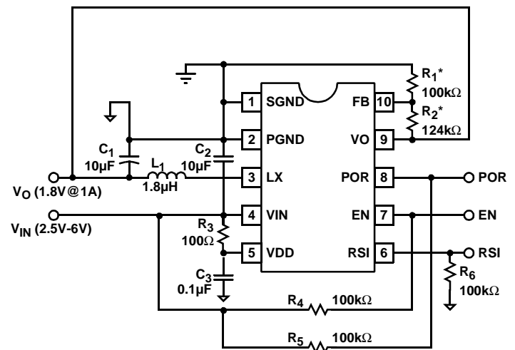
EL7536 TOP VIEW
