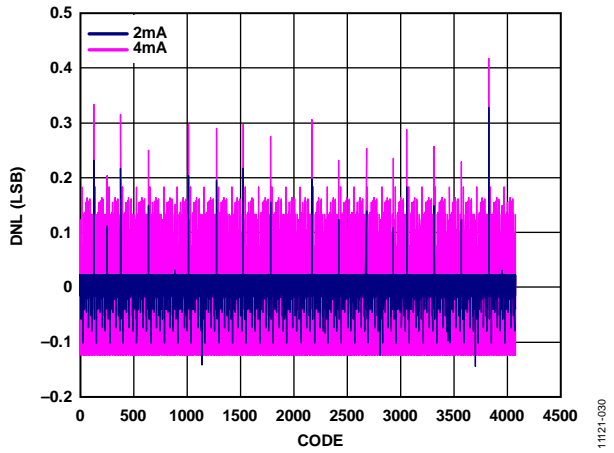
Figure 29. DNL, Three I_{OUTS} Values
