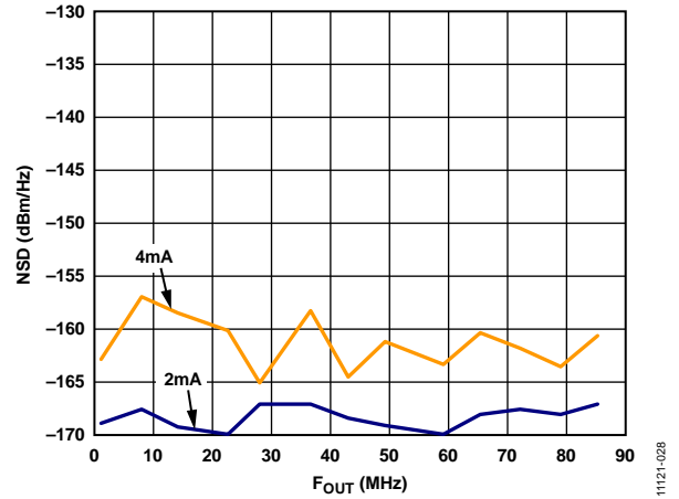
Figure 27. NSD vs. F_{OUT} , Two I_{OUTS} Values
