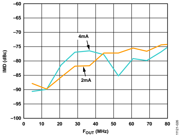
Figure 25. IMD vs. F_{OUT} , Two I_{OUTS} Values
