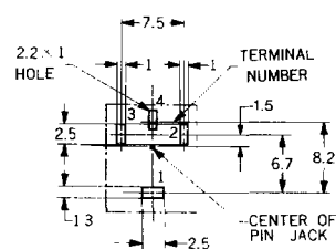
HOLE LAYOUT (BOTTOM VIEW)
