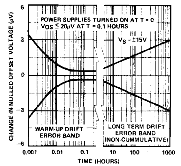
OFFSET VOLTAGE DRIFT WITH TIME
