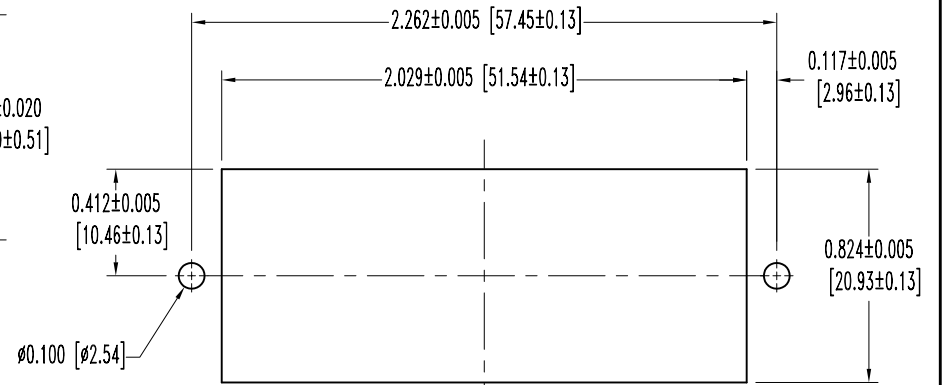
PANEL CUTOUT
