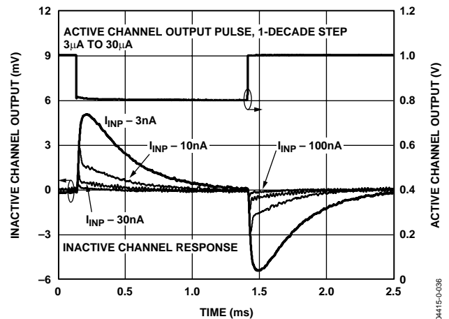
Figure 36. Crosstalk Pulse Response for Various Input Current Values
