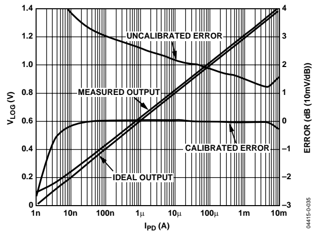
Figure 35. Using 2-Point Calibration to Increase Measurement Accuracy
