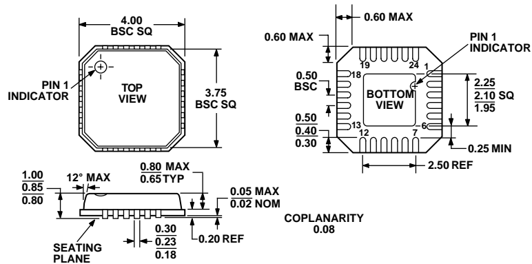
Figure 43. 24-Lead Lead Frame Chip Scale Package [LFCSP] (CP-24) Dimensions shown in millimeters
