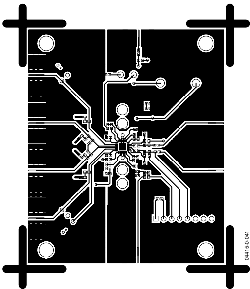
Figure 41. Component Side Layout
