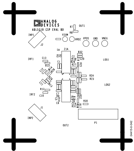
Figure 42. Component Side Silkscreen
