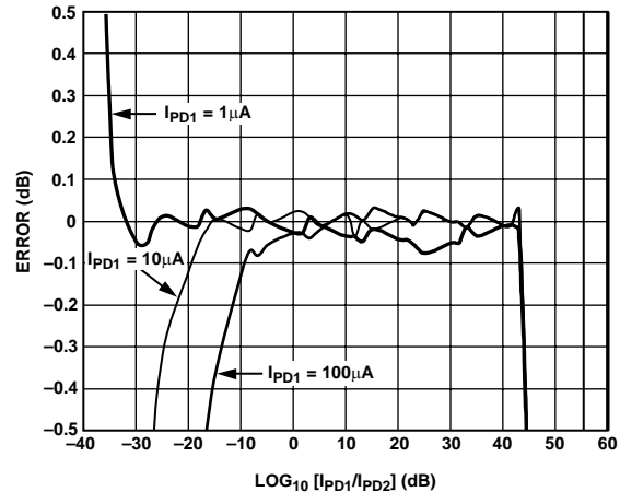
Figure 39. Log Conformance for Wilson Mirror ADL5310 Combination, Normalized to 10 mA Channel 1 Input Current, I_{IN1}
