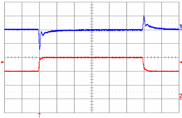
Fig. 1.0V.9: Output voltage response to load current step-change (20 A – 30 A – 20 A) at V_{in} = 48\text{ V} . Top trace: output voltage (100 mV/div.). Bottom trace: load current (10 A/div). Current slew rate: 1 A/ \mu\text{s} . C_o = 470\text{ }\mu\text{F} tantalum + 1 \mu\text{F} ceramic. Time scale: 0.2 ms/div.
