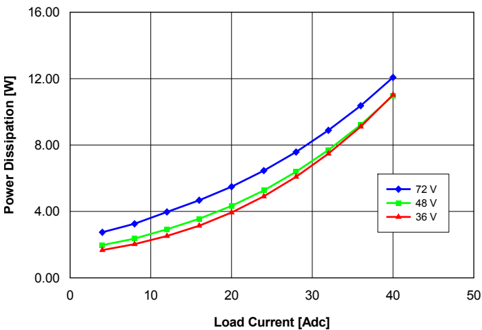
Fig. 2.0V.5: Power dissipation vs. load current and input voltage for converter mounted vertically with air flowing from pin 3 to pin 1 at a rate of 300 LFM (1.5 m/s) and T_a = 25\text{ }^\circ\text{C} .
