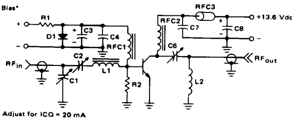
FIGURE 1 — COMMON-EMITTER TEST CIRCUIT
