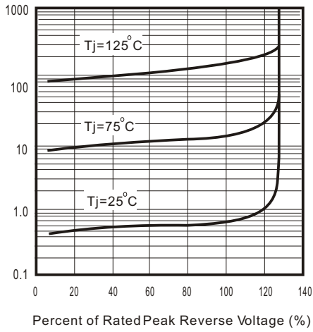
Fig. 1 - Reverse Characteristics
