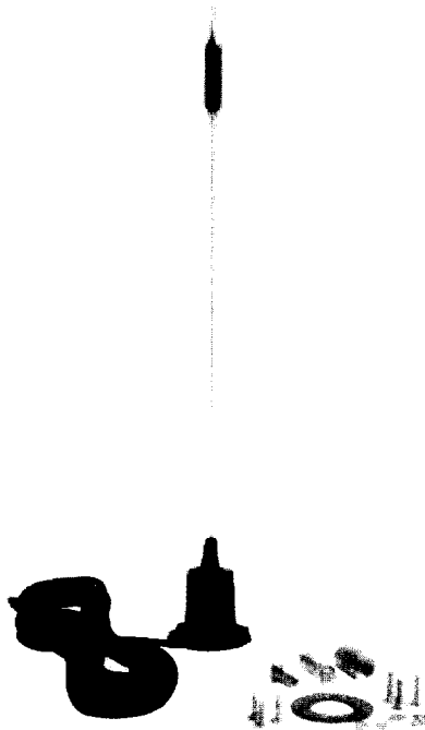
Complete self mounting UHF NGP antenna with pre installed coax and whip, 406-512 MHz
