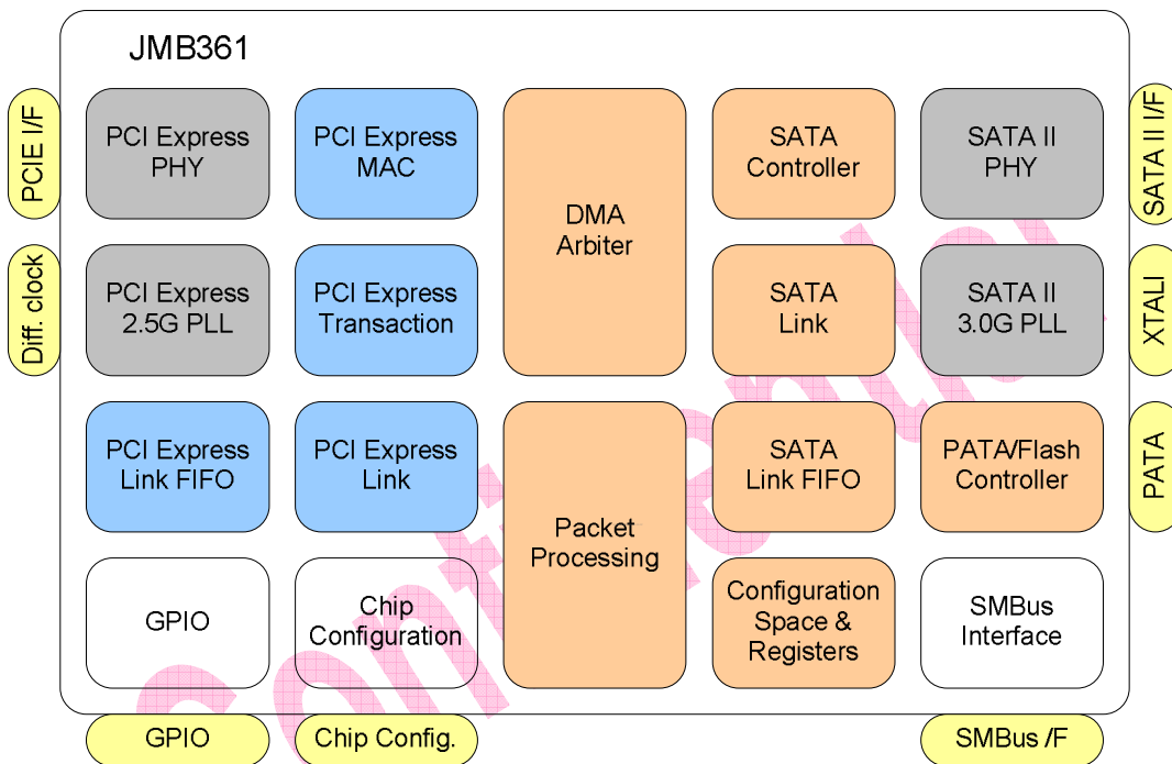
Functional Block Diagram of JMB361
